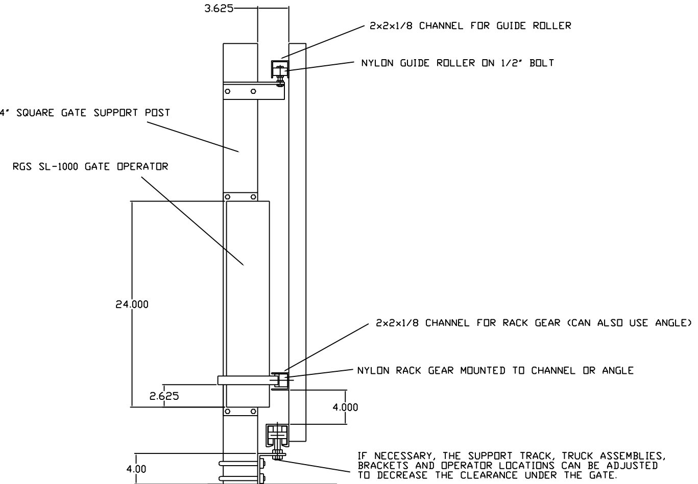
SL-1000 GATE PROFILE (GATE DESIGN AND DIMENSIONS MAY VARY)
